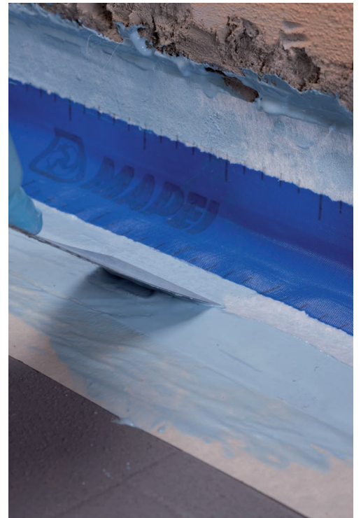
Application of Mapeband to a wall-floor joint with Mapelastc AquaDefense
