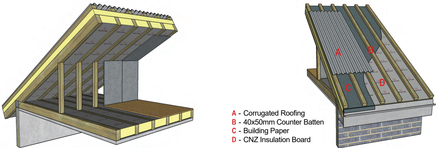
Figure 8.1. Pitched Roof Insulation
