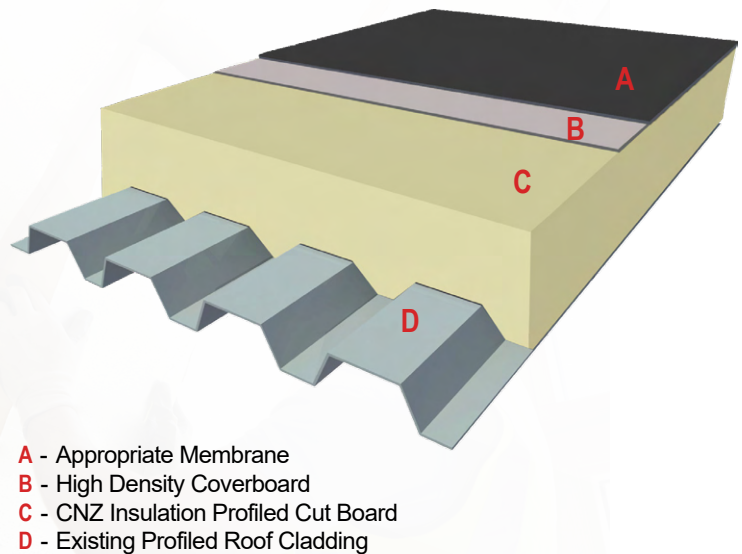
Figure 5.1. Profiled Cut Roof Insulation
