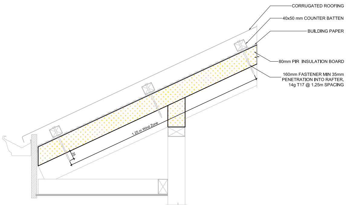
Figure 8.2. Eave Detail
