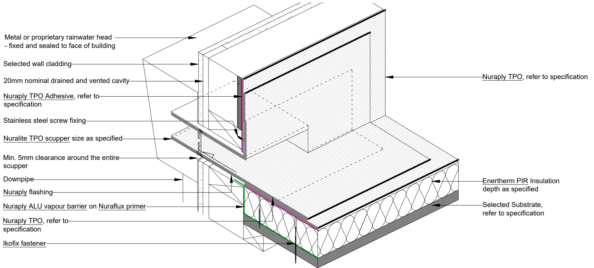
ISOMETRIC VIEW
